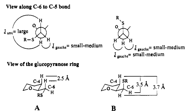
Figure 9. Two possible rotamers about the C-6–C-5 bond of sucrose dithiol (R = H) or sucrose disulfide (R = SR') and the resulting coupling constants. The distance between H-4 and H-6 in each rotamer is taken from the crystal structure of sucrose.
