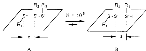
Figure 1. Equilibrium constant for thiol-disulfide interchange depends strongly on the C-S-S-C dihedral angle of the participating groups. Assuming that R_1 = R_2 = R_3 , that steric interactions between the R groups have no influence on K , and that the change in the CSSC angle is 90^\circ (as shown), the equilibrium constant K is 10^5 .
