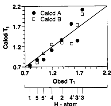
Figure 8. Comparison of the experimentally derived values of T_1 (s) with the calculated values of T_1 (s) for conformers A and B (Figure 7). The straight line is T_1(\text{calcd}) = T_1(\text{obsd}) . Deviations from this line indicate disagreement between observed and calculated values.
