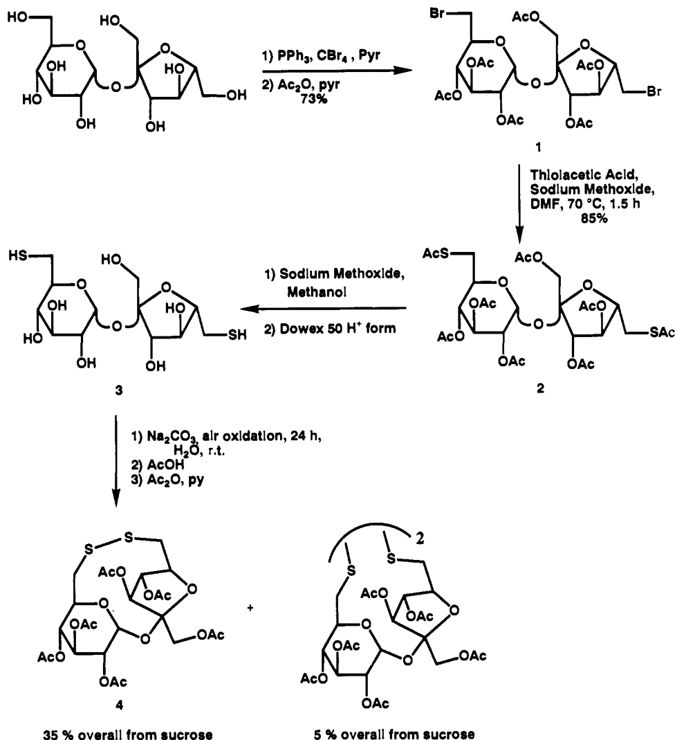
Scheme I. Synthesis of Sucrose Disulfide 4
