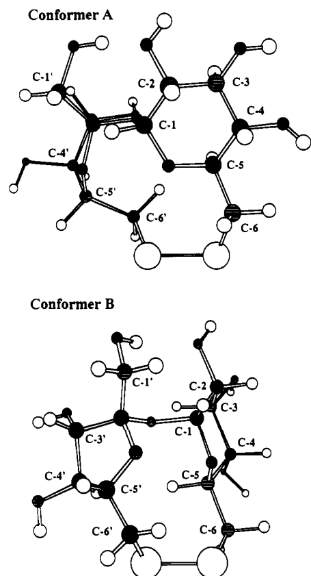
Figure 7. Structures of sucrose disulfide minimized by force field calculations. The CSSC angle in conformer A is 118^\circ ; that in conformer B is 96^\circ .
